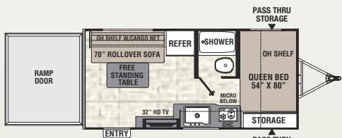
17 BLSE / Exterior Length 20' 4"
