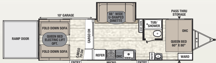
301 BLDS / Exterior Length 33' 7"
