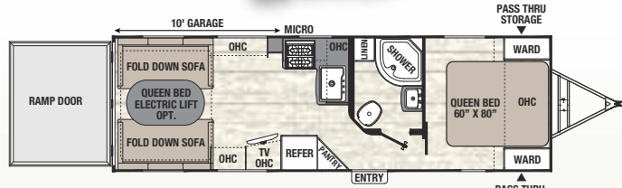
271 BL / Exterior Length 30' 11"
